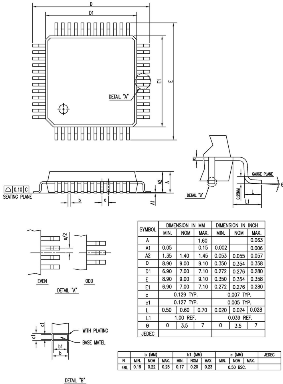
Figure 11-1 Outline Diagram of LQFP48 (7x7mm)
