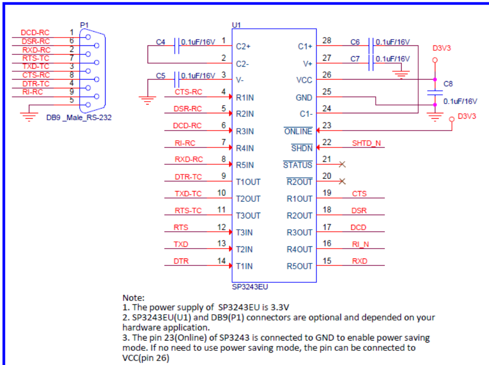
Figure 5-1 USB to RS232 Converter Example
