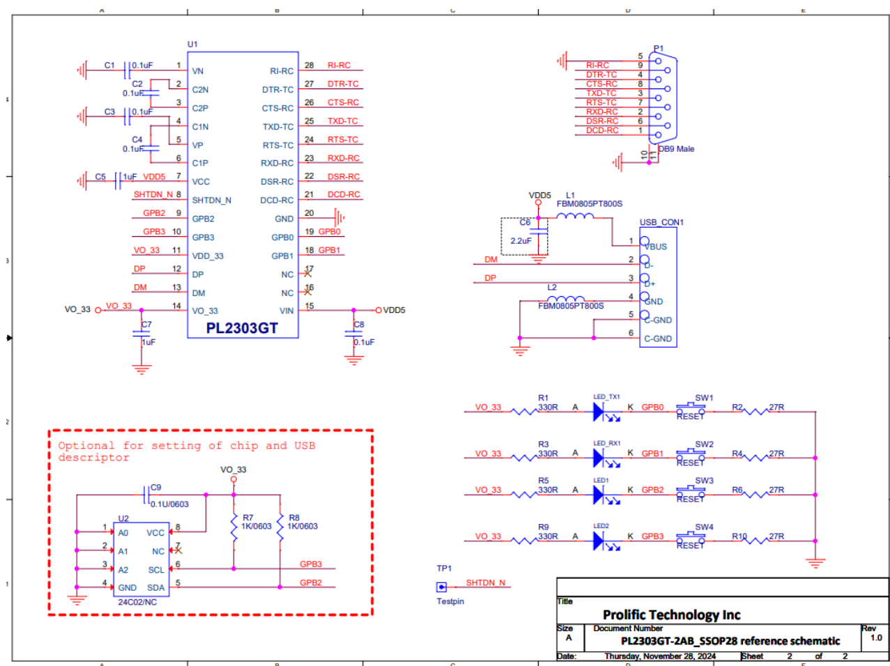
Figure 10-1 USB to RS232 Design Example
