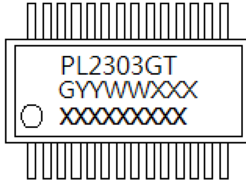
Figure 12-1 Chip Part Number Information (SSOP)
