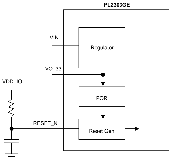
Figure 10-3a Chip Reset Control Application
