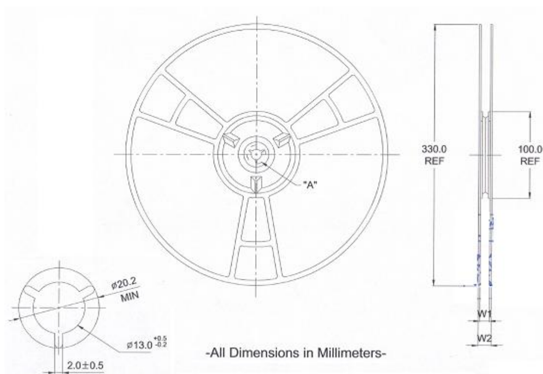
Figure 13-2 Reel Dimension
