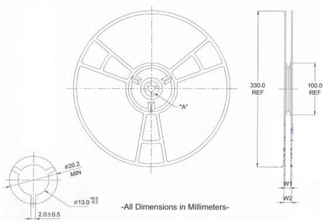
Figure 13-2 Reel Dimension
