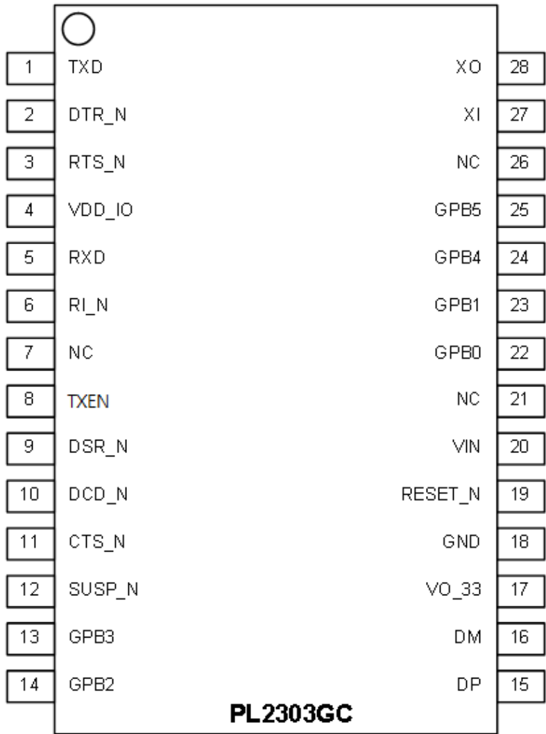
Figure 7-1 PL2303GC Pin Diagram (SSOP28)
