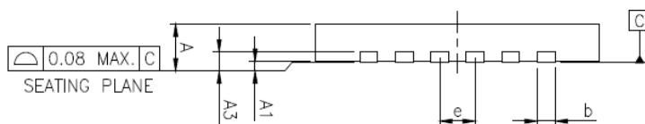
SIDE VIEW
