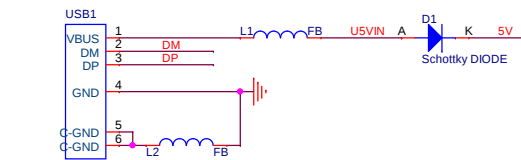
USB TYPE B
