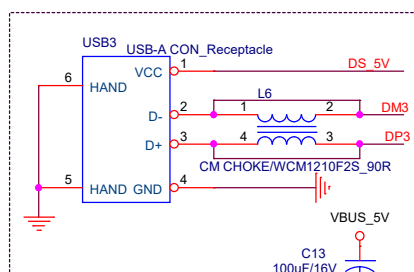
Device Port3
