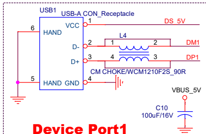
Device Port1
