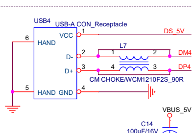
Device Port4
