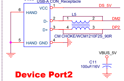
Device Port2
