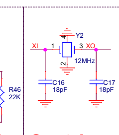
Crystal
