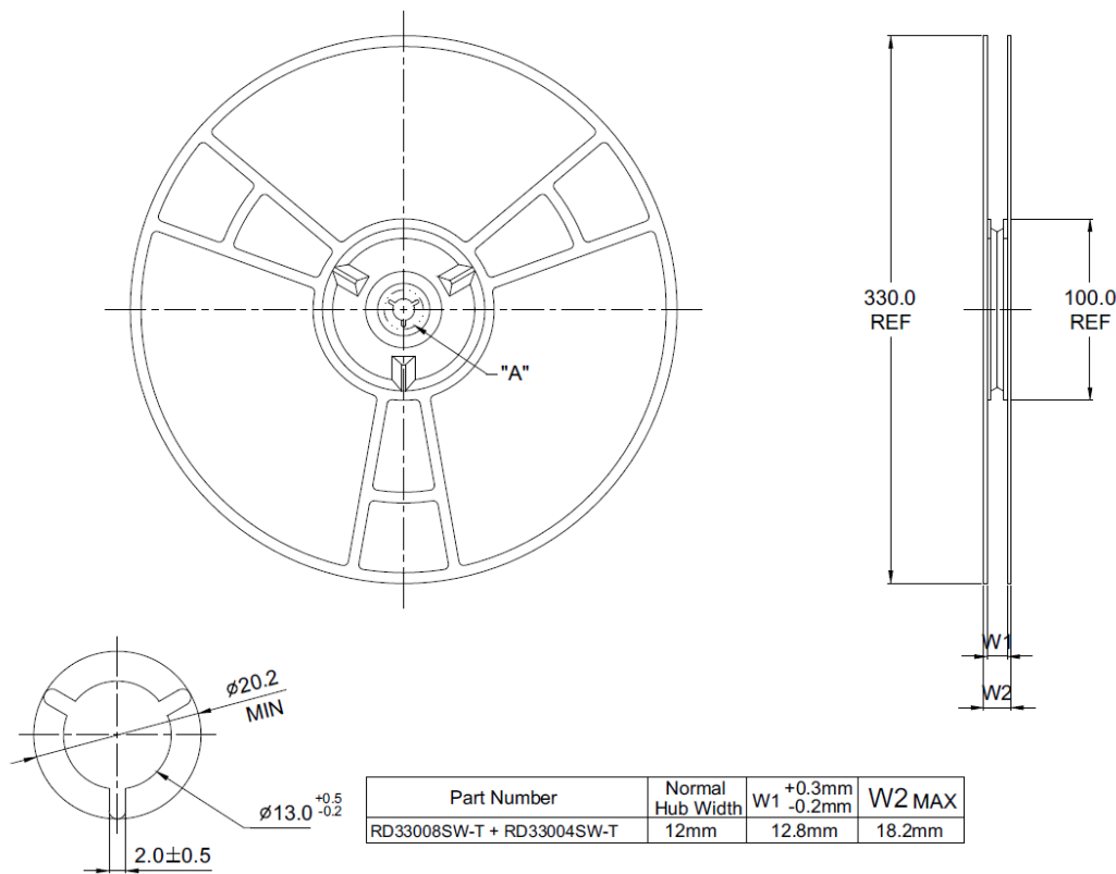
Figure 8-2: Reel Dimension
