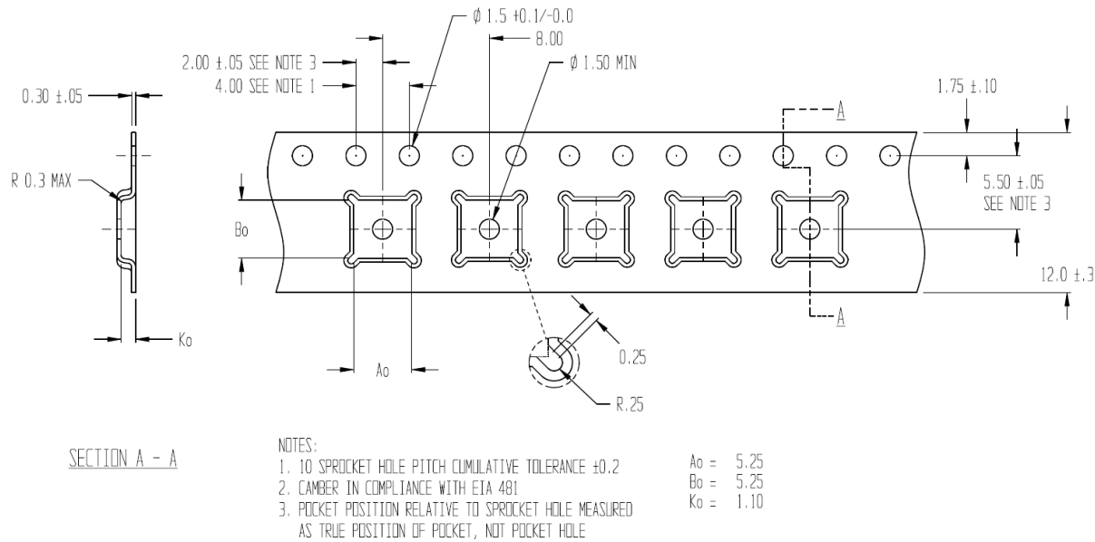
Figure 8-1: QFN32Carrier Tape
