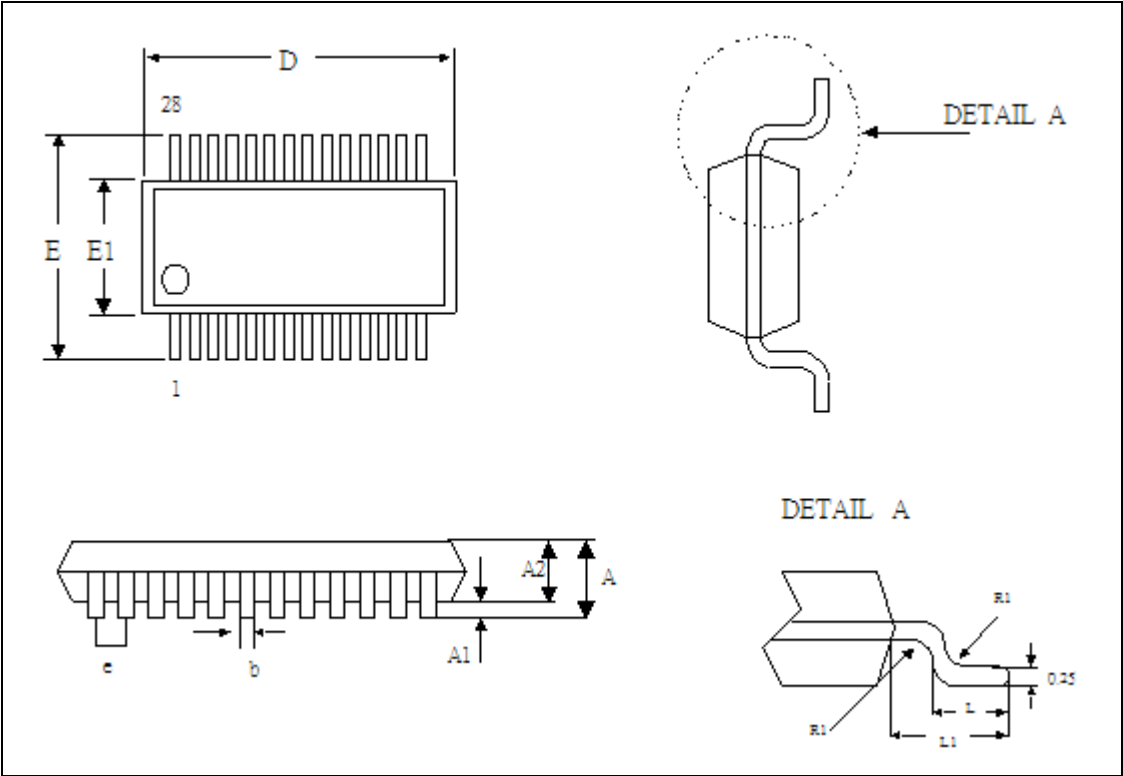
Figure 12-2 PL2303GT Outline Diagram (SSOP28)
