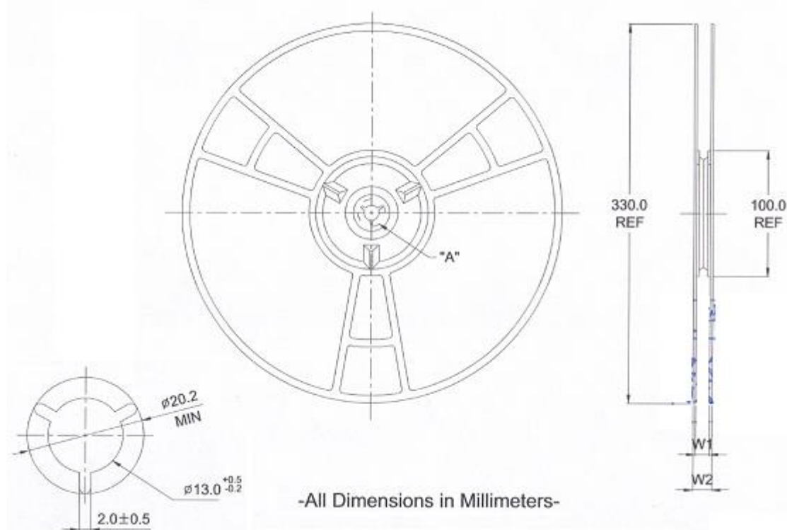
Figure 13-2 Reel Dimension
