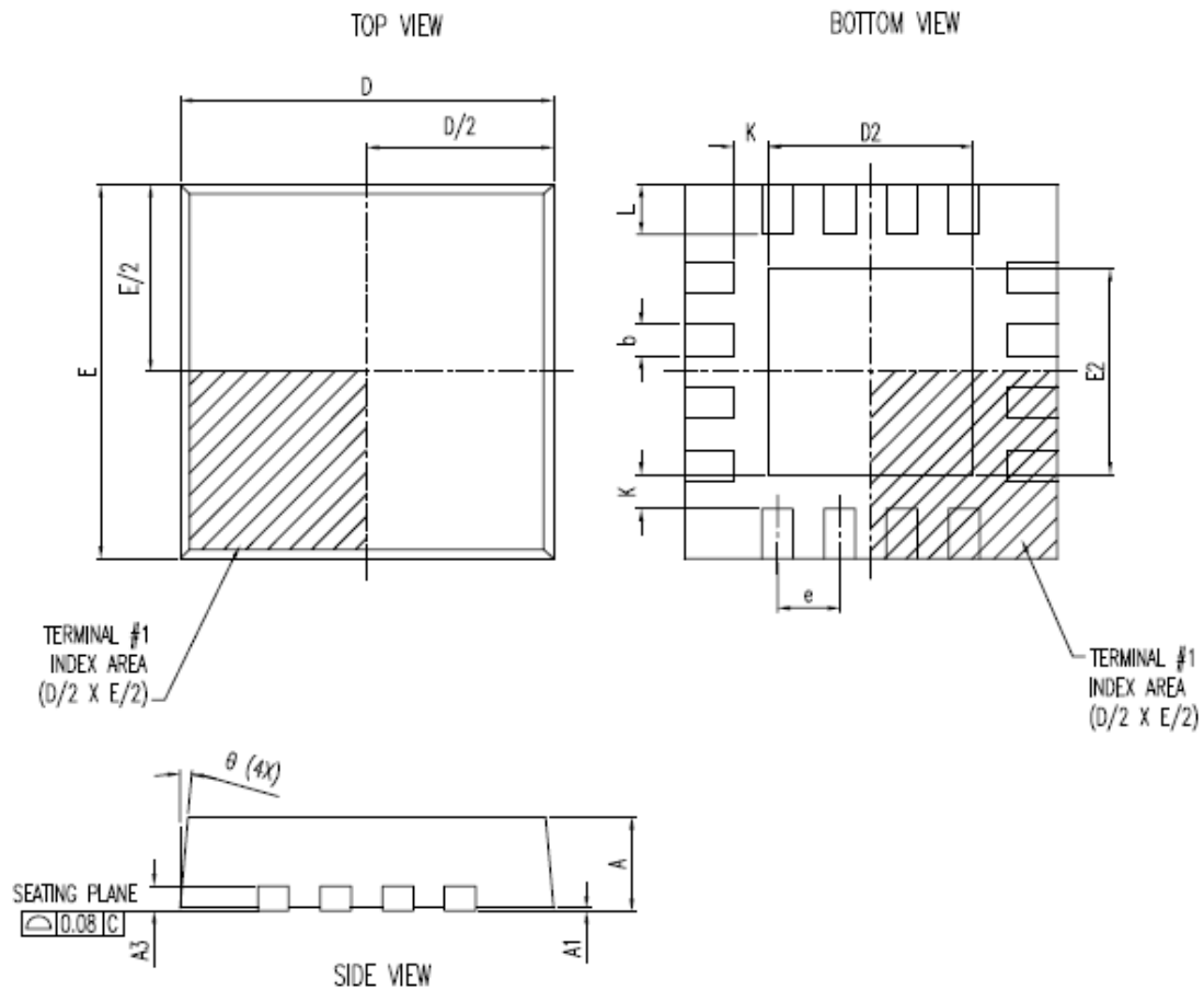
Figure 12-1 PL23C3 Outline Diagram (QFN16)
