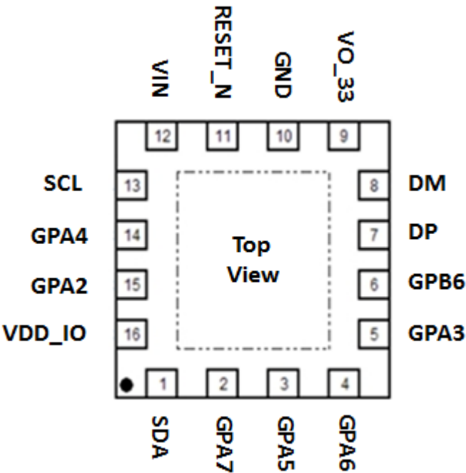
Figure 7-1 PL23C3 Pin Diagram (QFN16)
