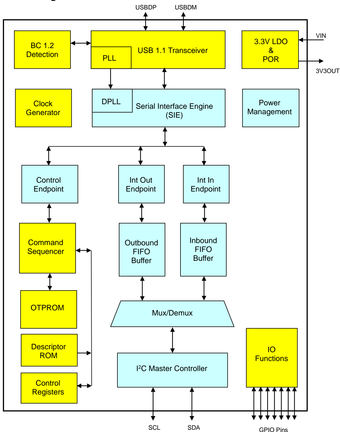
Figure 4-1 PL23C3 Block Diagram
