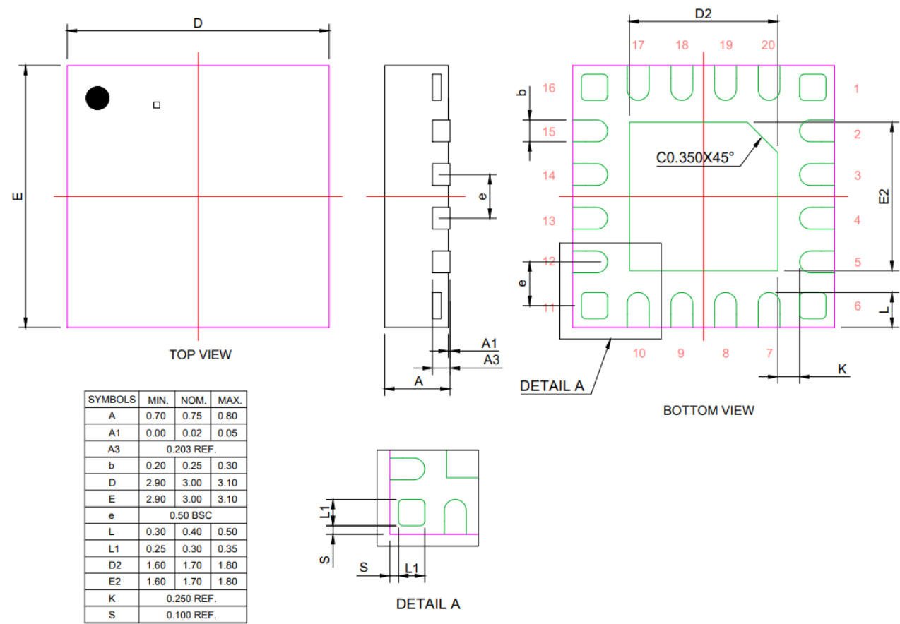
Figure 12-3 PL2303GC Outline Diagram (QFN20) 3 x 3 mm
