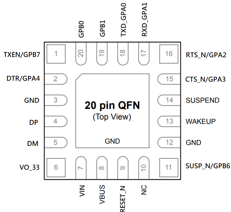
Figure 7-3 PL2303GC Pin Diagram (QFN20)
