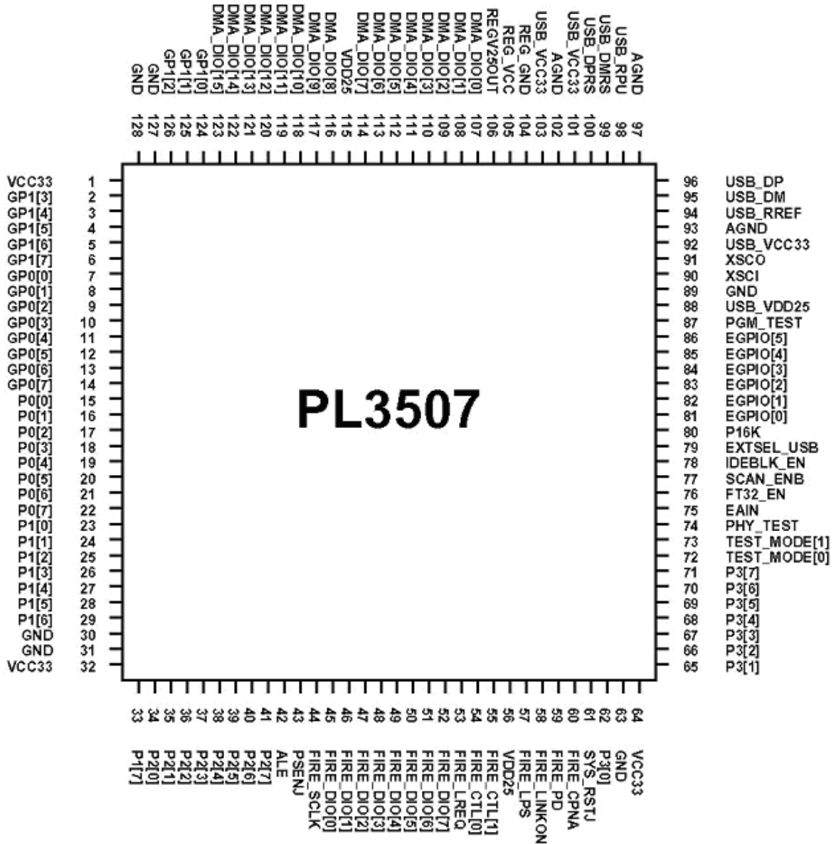
Figure 5-1 Pin Assignment Outline of PL-3507 (Chip Rev D)
